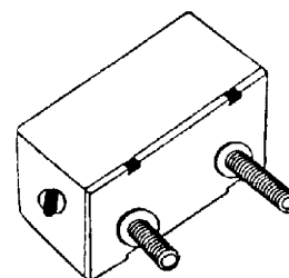
CIRCUIT BREAKER 12-VOLT MANUAL RESET TYPE 3 50 AMP CRV# 442944 15 AMP CRV #442945 30 AMP CRV #413544 40 AMP CRV #471191
